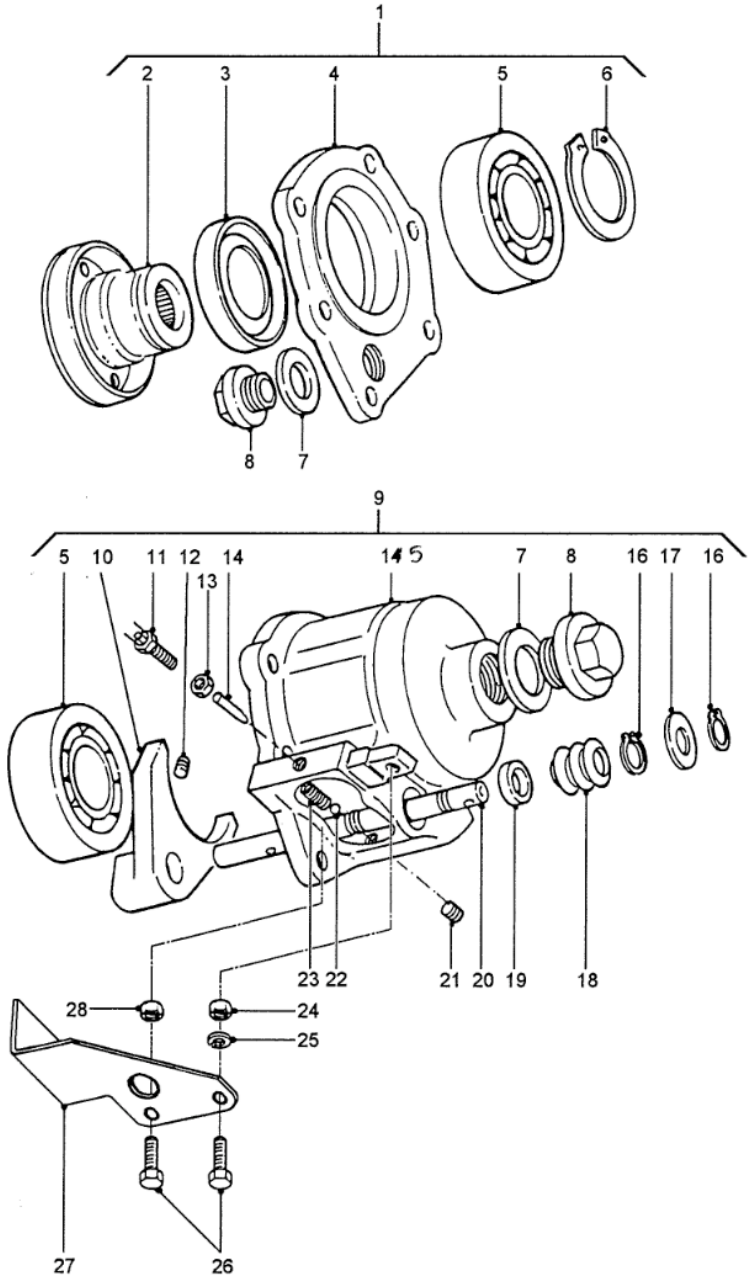
POWER TAKE - OFF BEARING & SELECTOR HOUSING ASSEMBLIES
