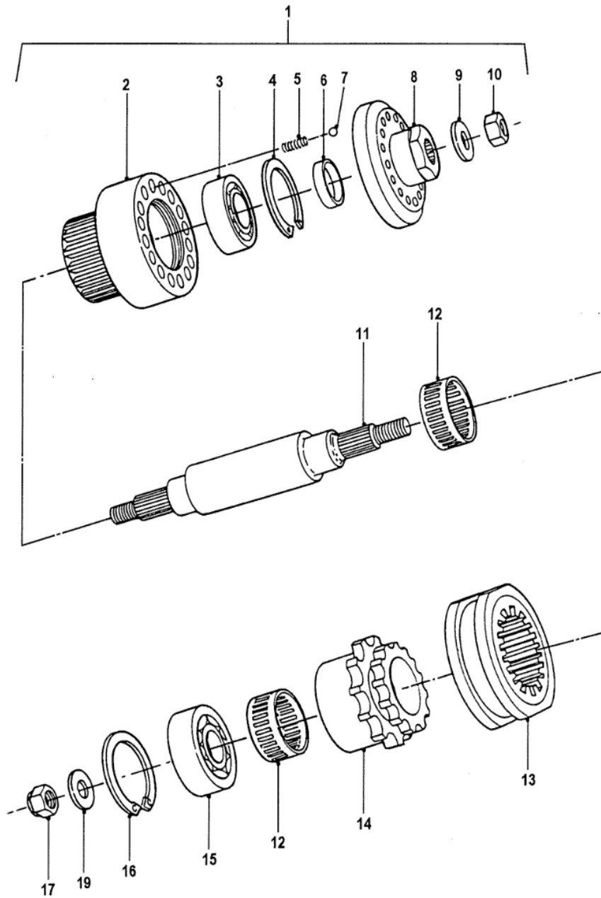
POWER TAKE - OFF AND TORQUE LIMITER
