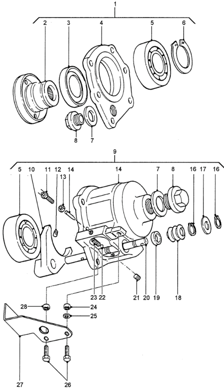
POWER TAKE - OFF BEARING & SELECTOR HOUSING ASSEMBLIES
